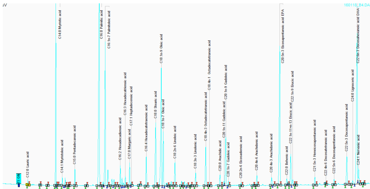
Complete chromatogram.
