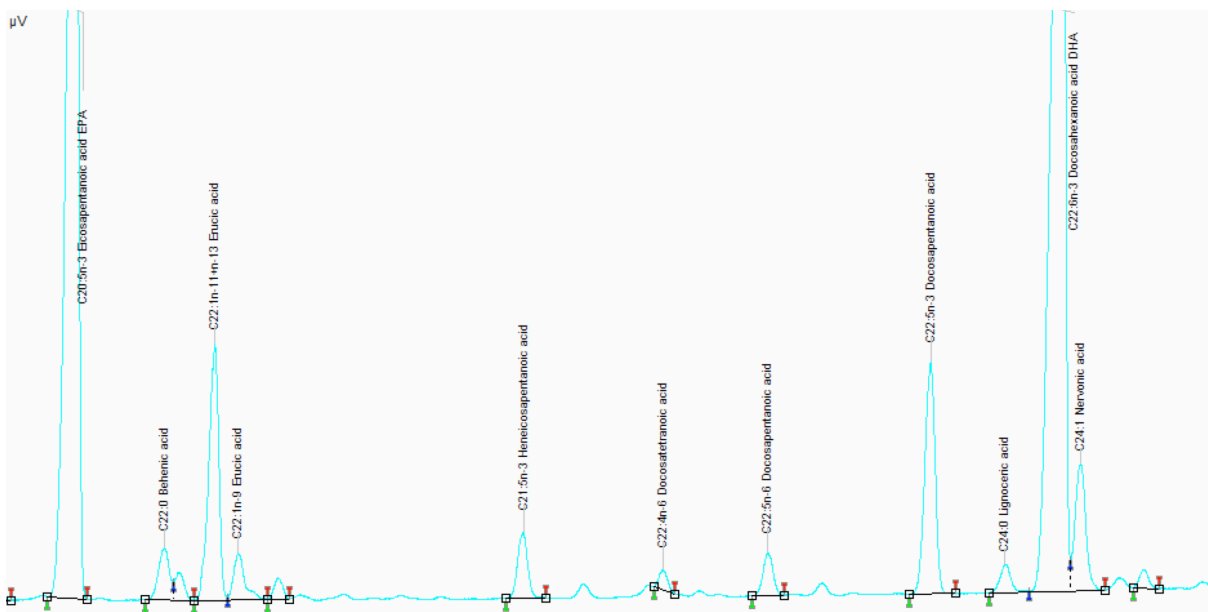
C20:5 - C24:1 Section.
