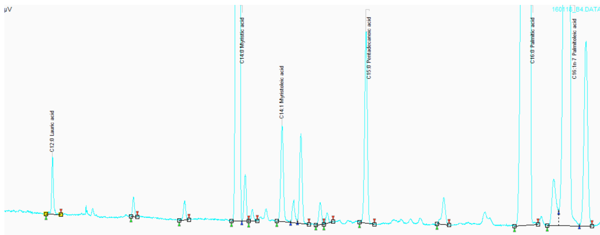
C12:0 to C16:1 section.
