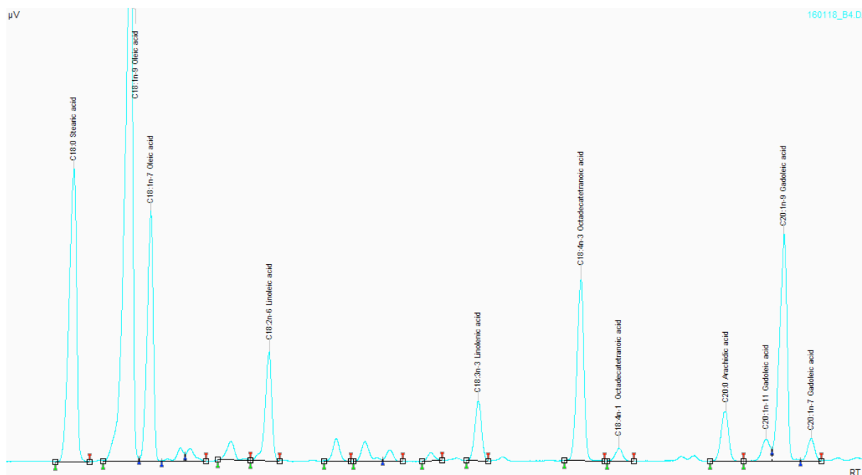
C18:0 – C20:1 section.
