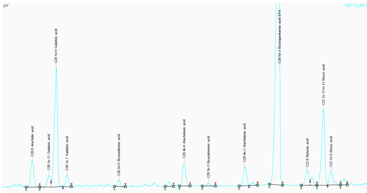
C20-C22:1 Section
