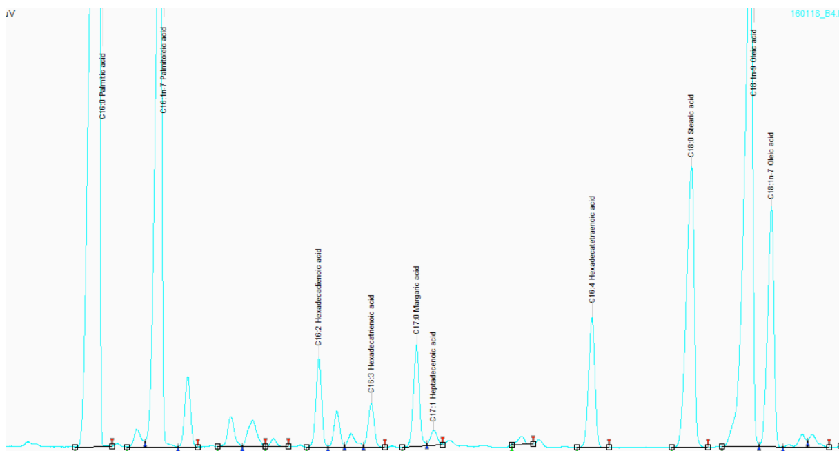
C16:0 – C18:1 section. (small peaks in the middle is a challenging area, may be deviations)
